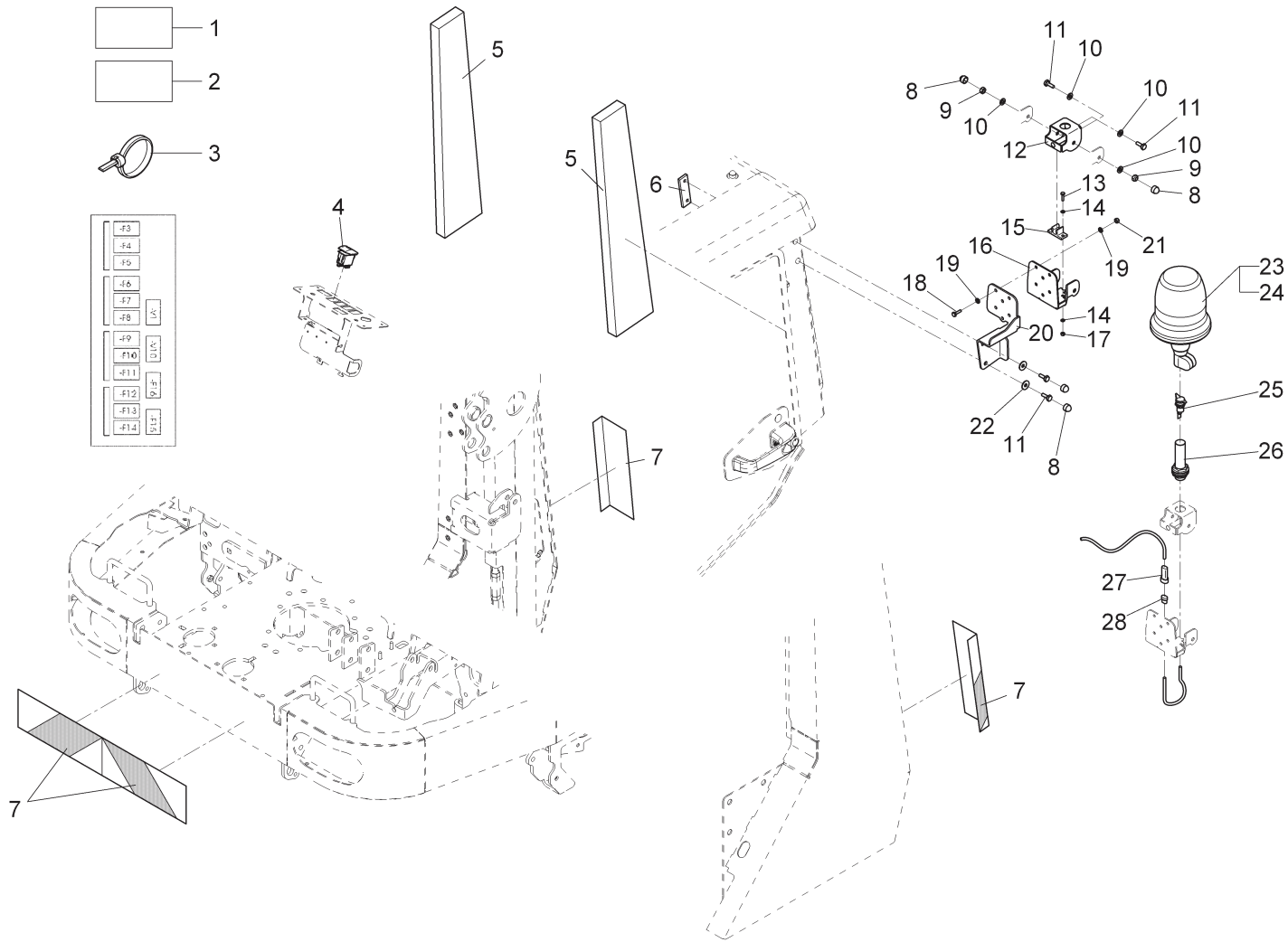
Fig.1 Assembly drawing
